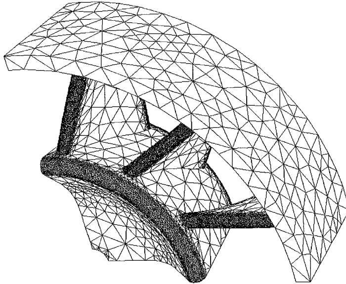
Figure 13. Optimized mesh of a mechanical device
