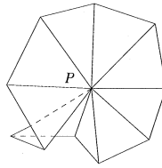
Figure 1. Vertex P is a non-conforming vertex
