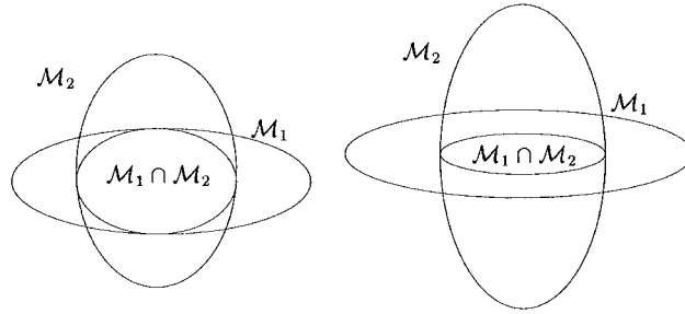
Figure 4. Metric intersection. Left: using the simultaneous reduction of \mathcal{M}_1 and \mathcal{M}_2 , right: preserving the direction of \mathcal{M}_1
