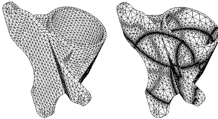
Figure 14. Adapted surface mesh, iterations 0 and 3
