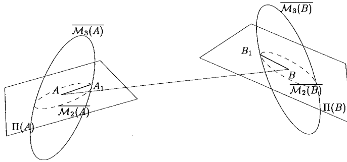
Figure 8. Definition of the metric \mathcal{M}_2 in the tangent planes \Pi(A) and \Pi(B) associated with points A and B
