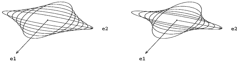
Figure 3. Metric interpolation. Left: linear interpolation, right: geometric interpolation
