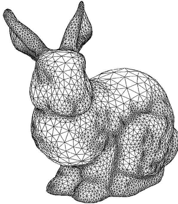
Figure 10. Simplified surface triangulation of Stanford bunny (gap 14^\circ )
