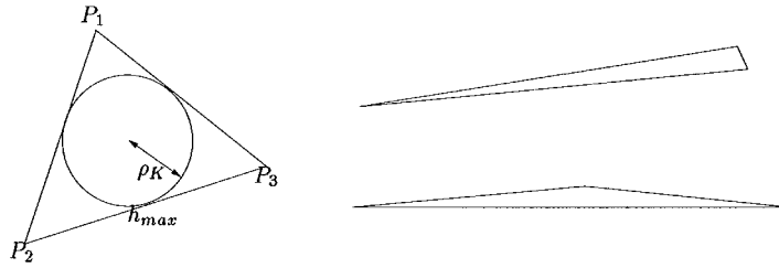
Figure 5. Triangle aspect ratio (isotropic case): well-shaped (left) and degenerated triangles (right)
