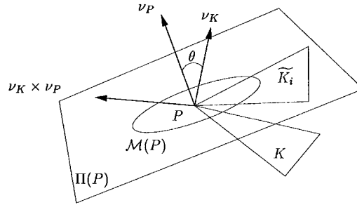
Figure 6. Shape quality of a surface triangle measured in the tangent plane \Pi(P) associated with vertex P ( \mathcal{M}(P) denotes the metric at P )
