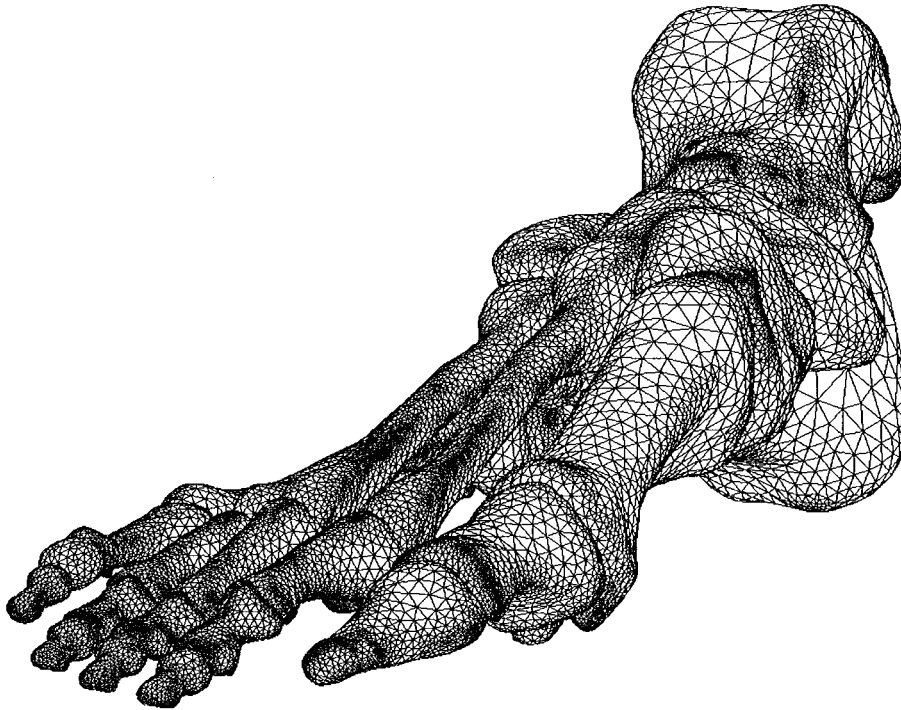
Figure 9. Optimized surface triangulation of a foot skeleton
