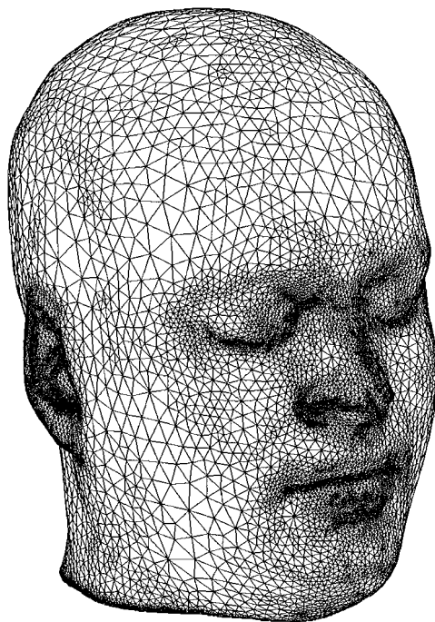
Figure 11. Optimized surface triangulation of a human head (gap 3^\circ )
