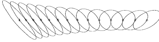
Figure 7. Geometric interpolation along a segment AB
