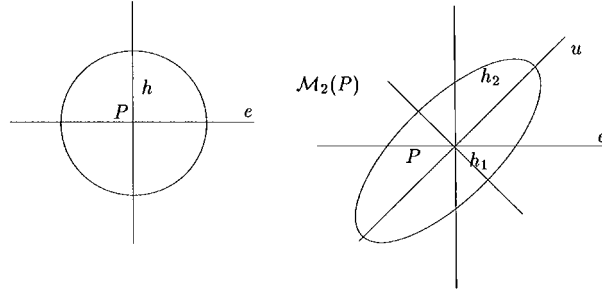
Figure 2. Geometric interpretation of a metric. Left: an isotropic metric corresponds to a circle, right: an anisotropic metric corresponds to an ellipse aligned with any arbitrary orthonormed vectors)
