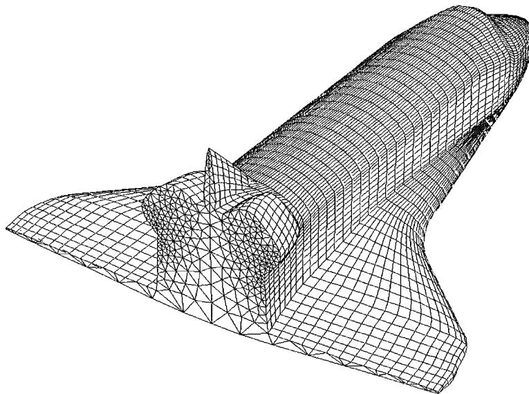
Figure 12. Surface triangulation of the Columbia shuttle
