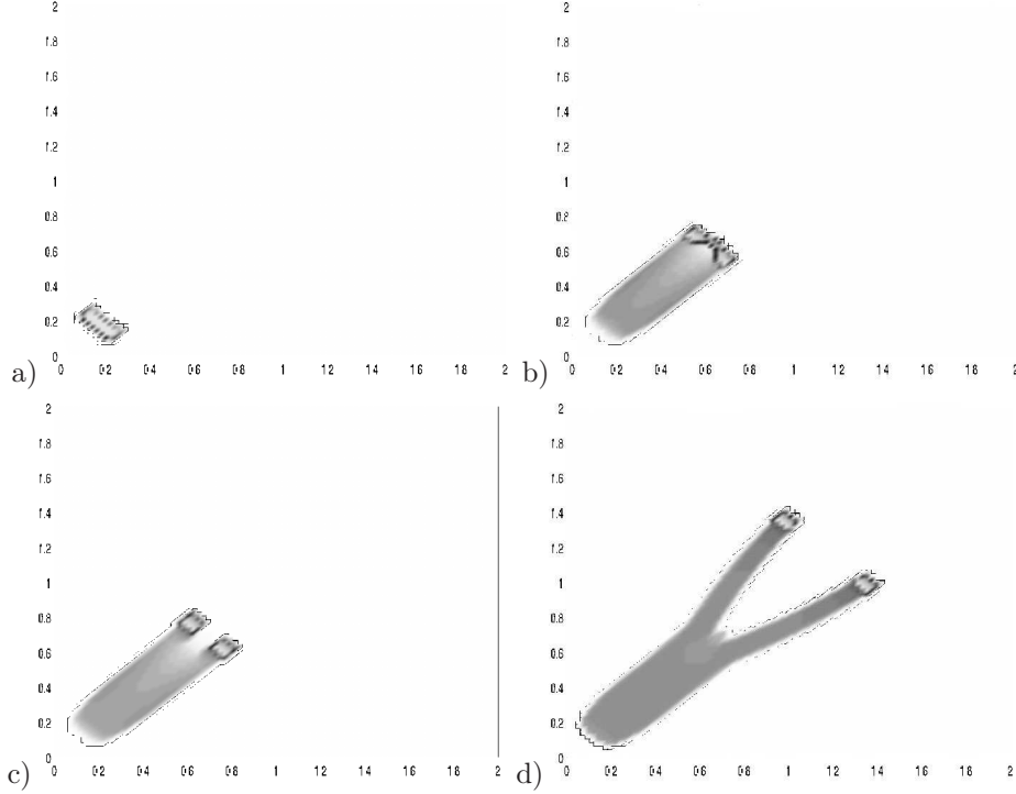
Figure 6. Time dynamic of swarms plus supporters density computed with the 2d model (4.3) with supporter cells.
